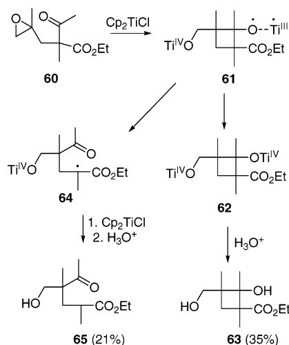
SCHEME 21. Reaction of Epoxide 60 with Ti(III)
